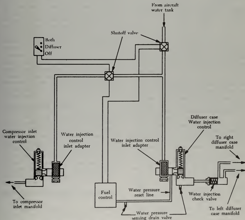
FIGURE 3-61. A typical water injection system.
